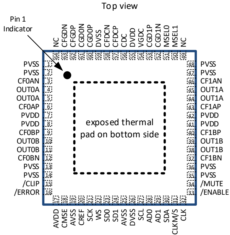
Figure 4-1 Pinout MA12070P
