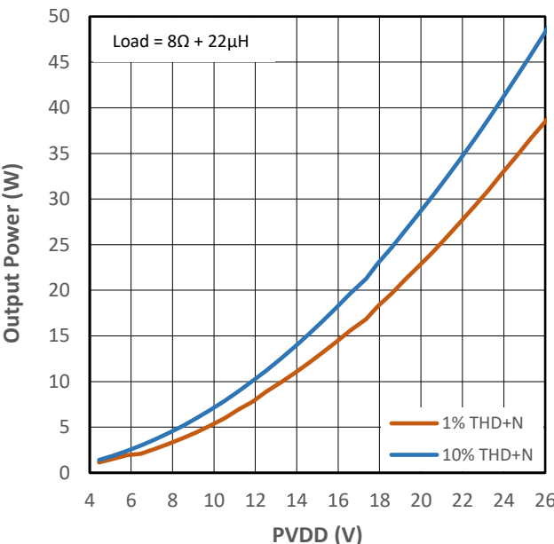
Figure 11-22 Output Power vs PVDD for PMP1
