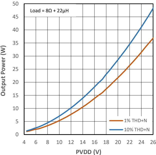
Figure 11-24 Output Power vs PVDD for PMP4
