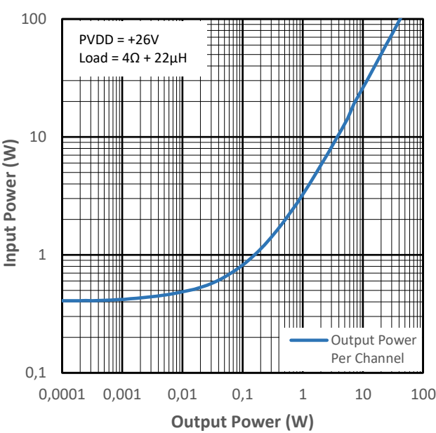
Figure 10-14 Input Power vs Output Power for PMP1
