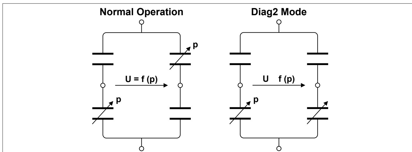
Figure 39 Diag2 functionality
