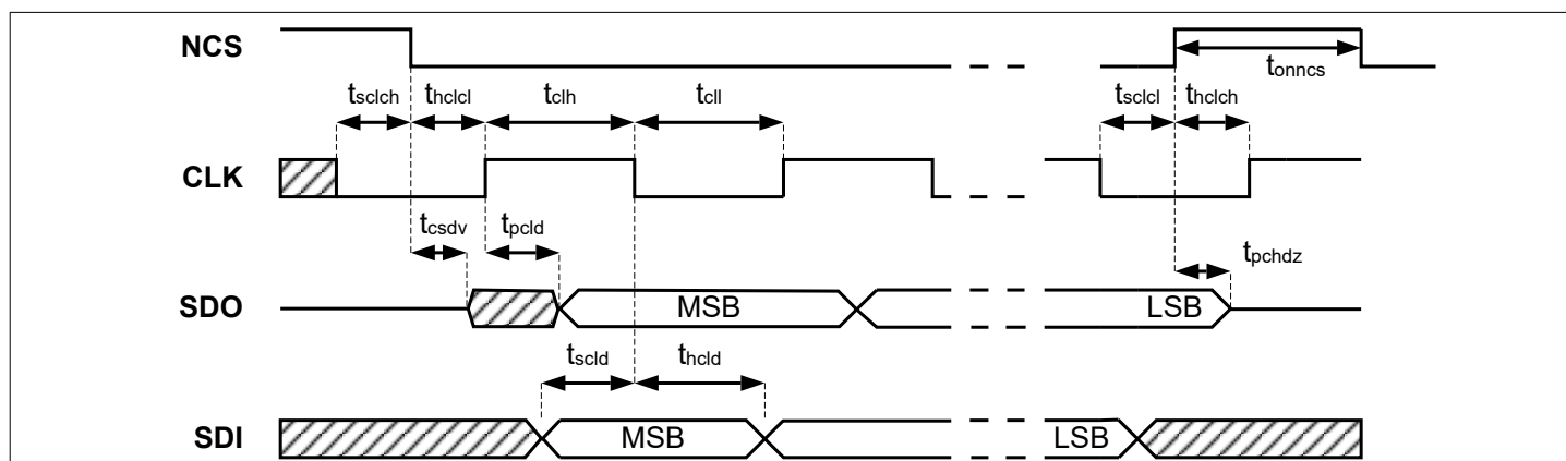
Figure 6 SPI timing
