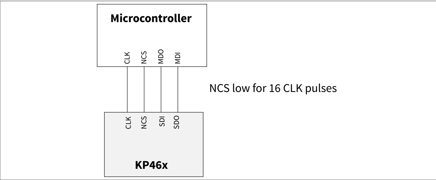
Figure 32 Example for single device operation The SPI signal timing for single device operation is shown in the figure below.
