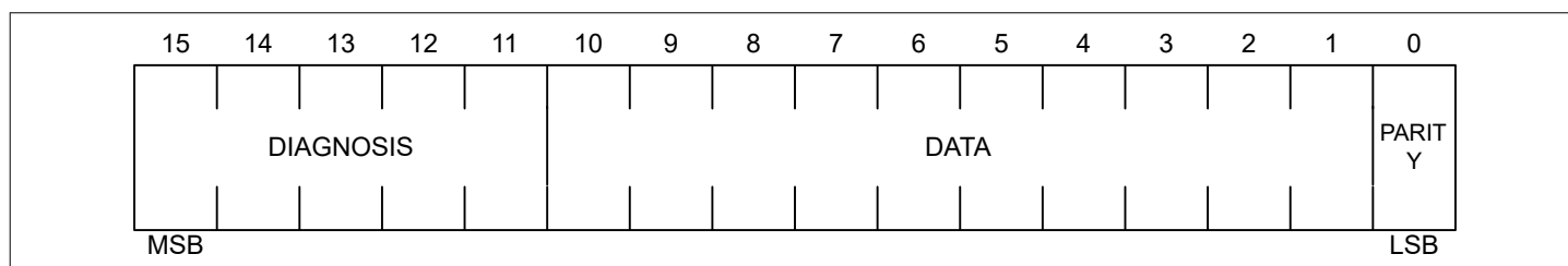
Figure 8 SPI response structure (10-bit)
