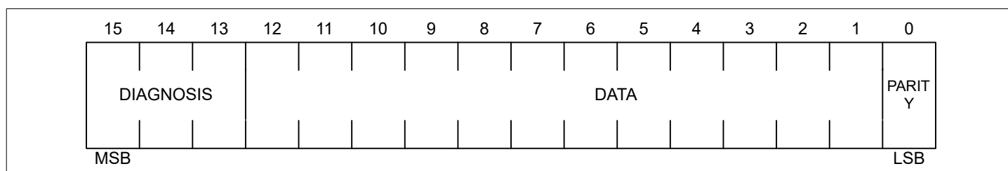
Figure 9 SPI response structure (12-bit)
