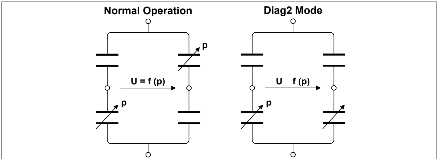
Figure 39 Diag2 functionality
