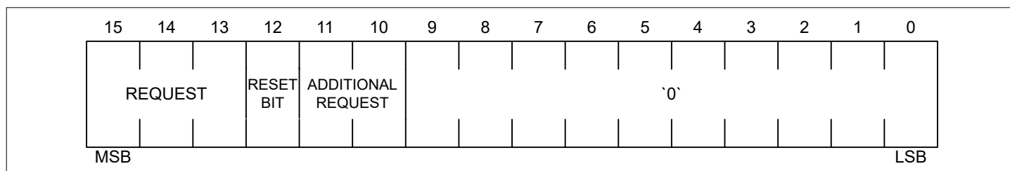
Figure 7 SPI command structure
