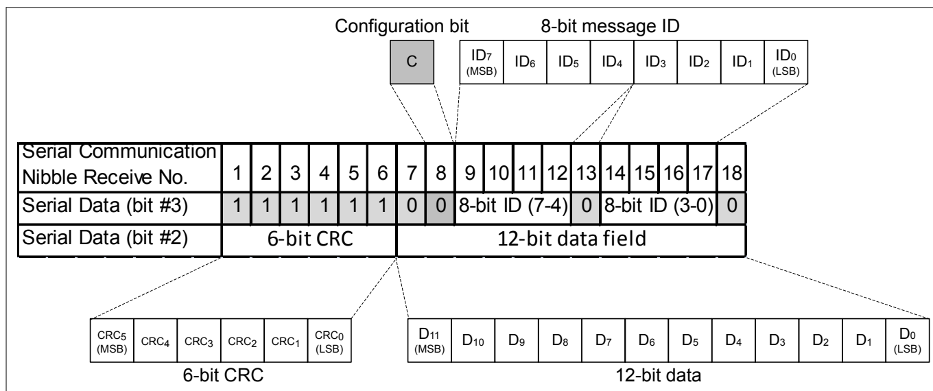
Figure 10 Enhanced serial message format with 12-bit data field and 8-bit message ID
