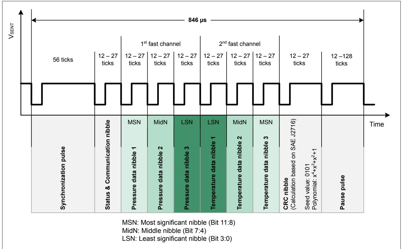
Figure 7 Message transmission
