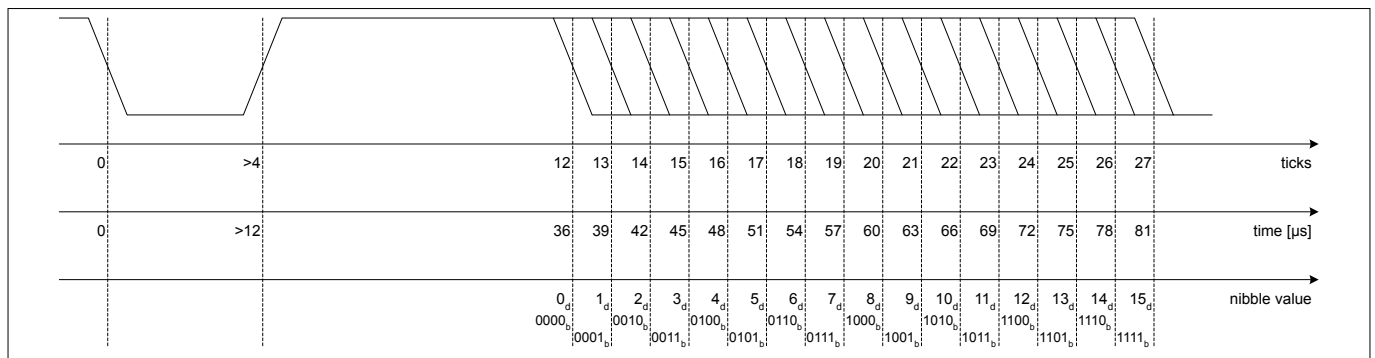
Figure 8 Nibble timing
