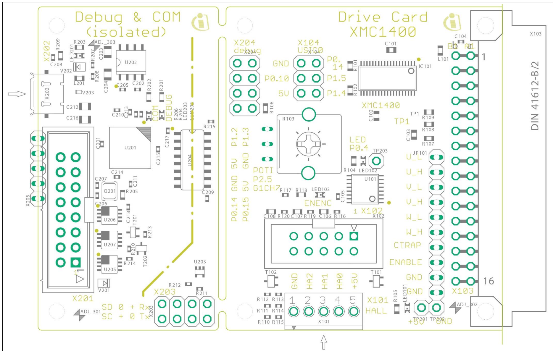
Figure 17 Component placement
