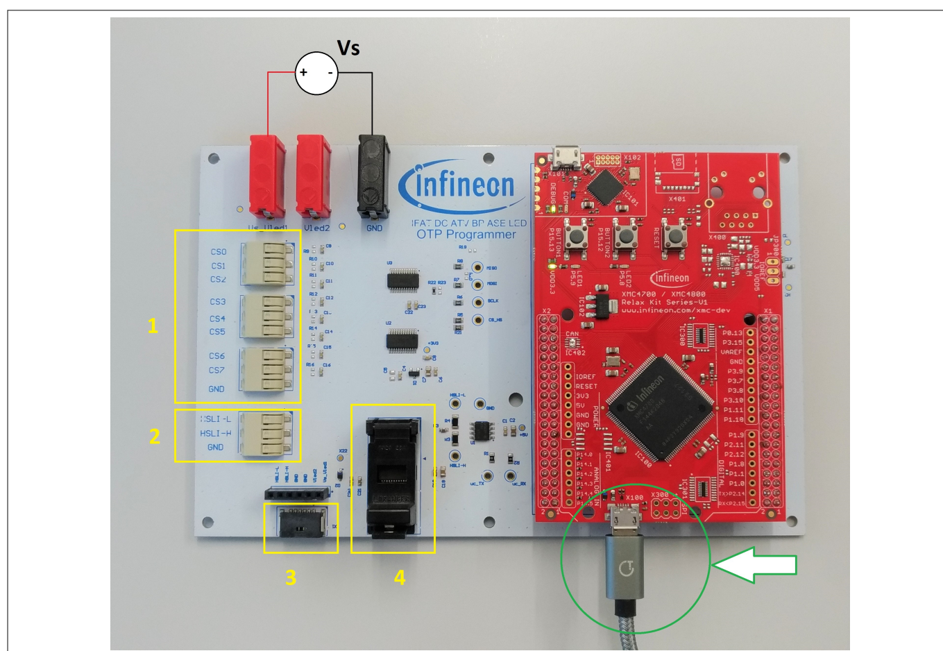
Figure 13 OTP programming setup connection
