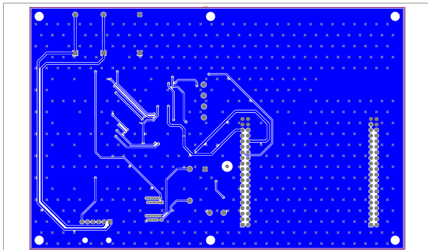
Figure 16 Bottom layout
