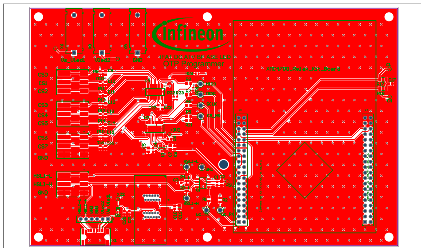
Figure 15 Top layout
