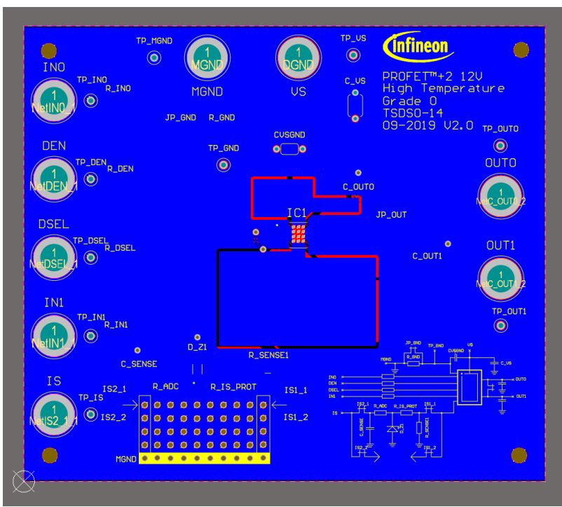
Figure 30 PROFET™ +2 12V Grade0 customer evaluation board bottom layout
