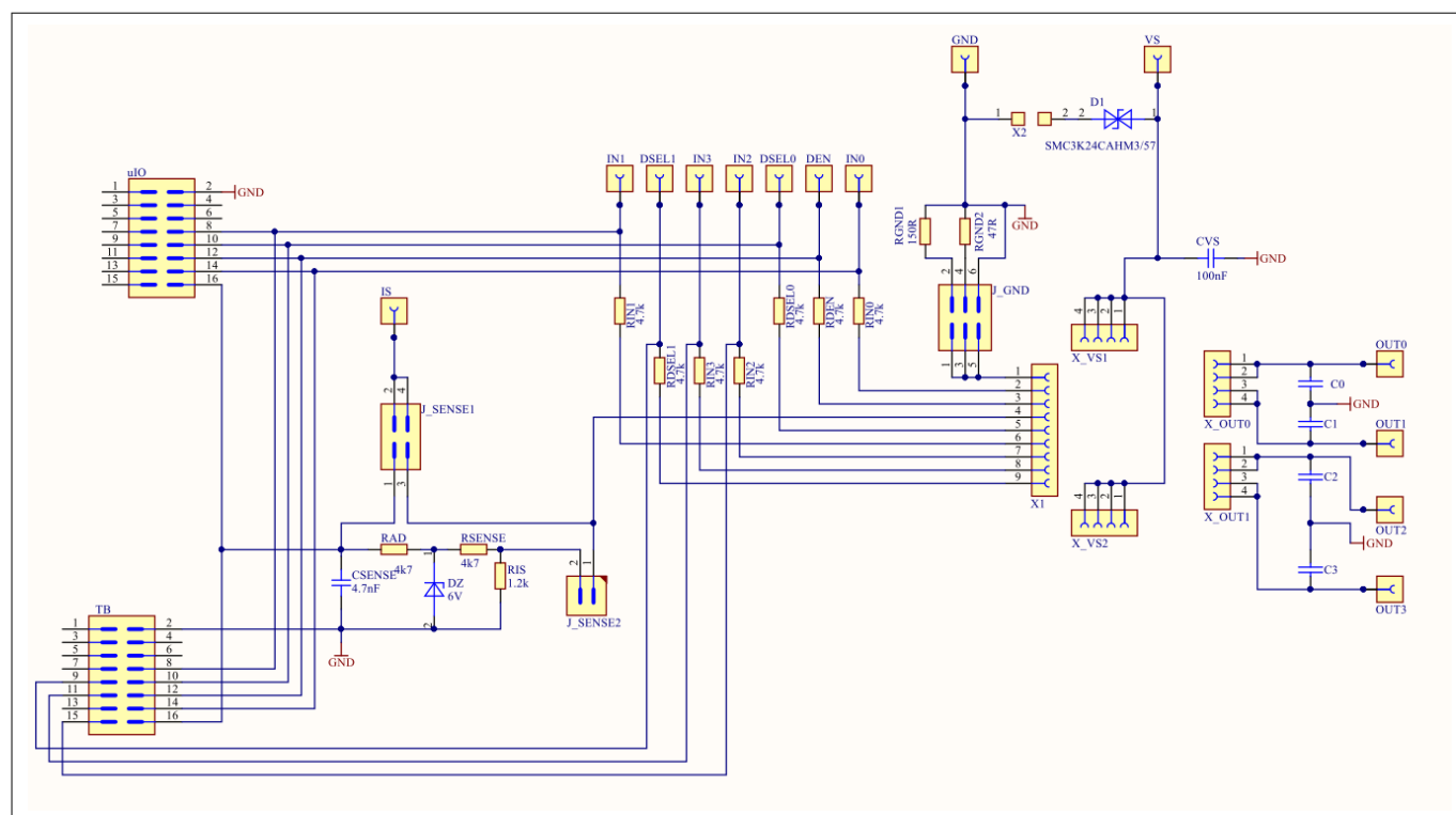
Figure 6 Motherboard V2.0 schematic
