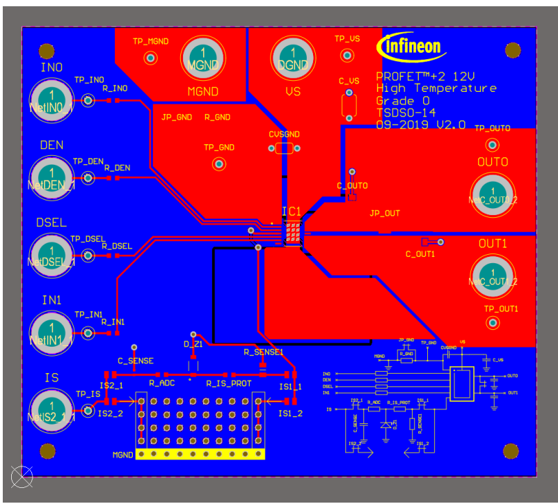
Figure 29 PROFET™ +2 12V Grade0 customer evaluation board top layout
