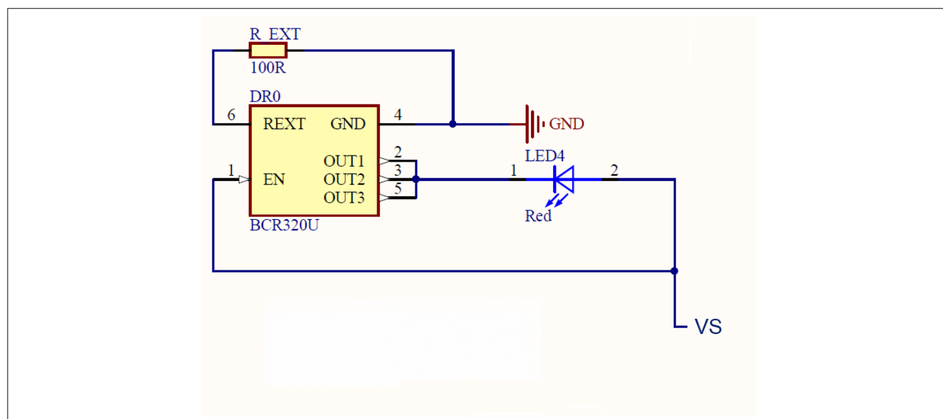
Figure 22 BCR320U circuit
