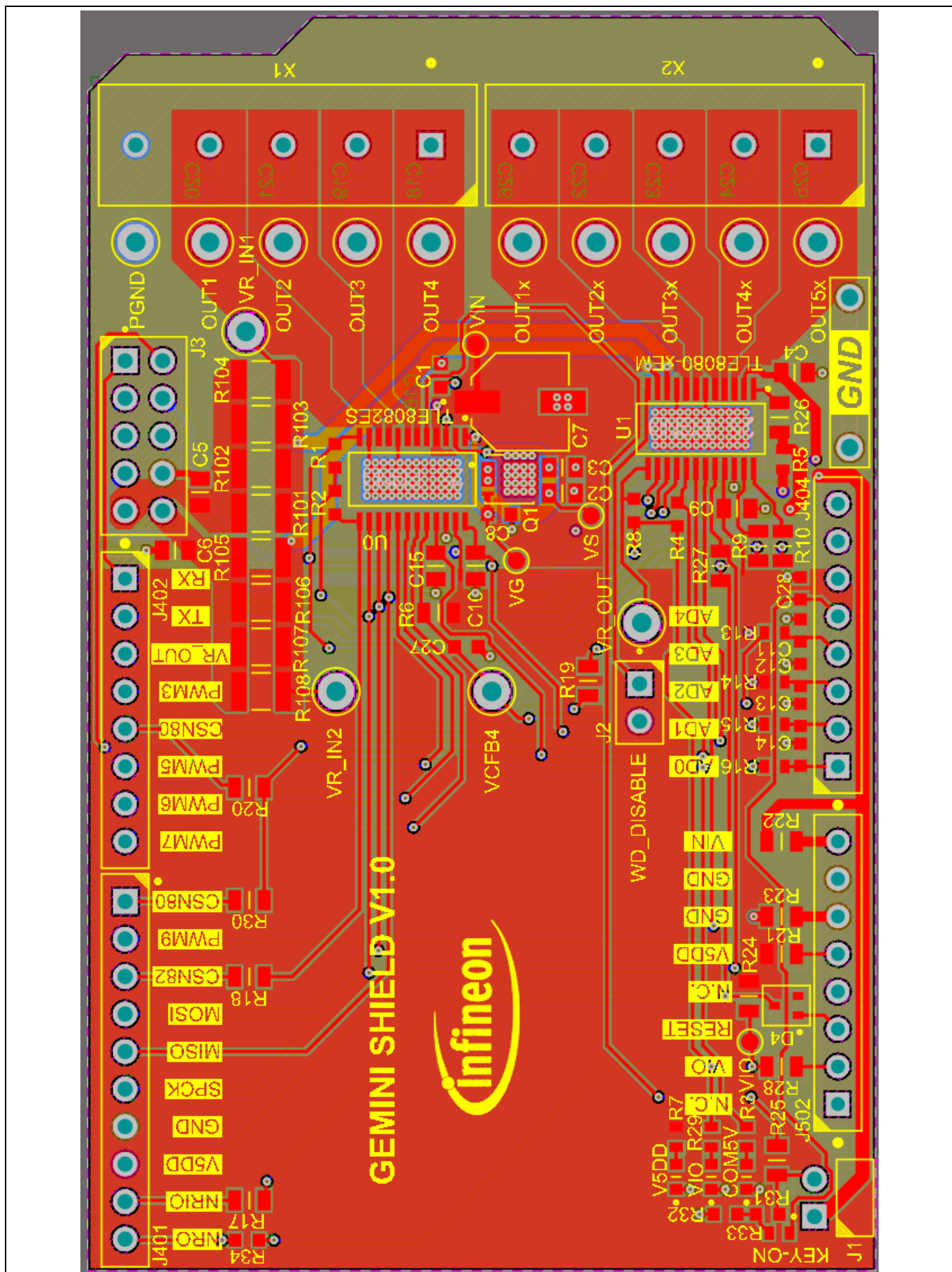
Figure 11 Layout Evaluation-PCB
