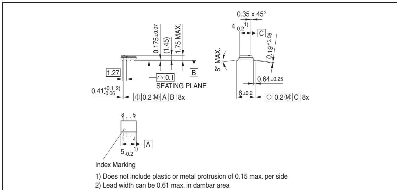
Figure 8 PG-DSO-8 1)
