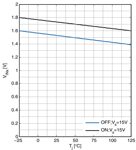
Input Threshold voltage V_{\text{INH,Lx}} versus Junction Temperature T_j
