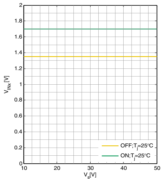
Input Threshold voltage V_{\text{INH,Lx}} versus Supply Voltage V_s
