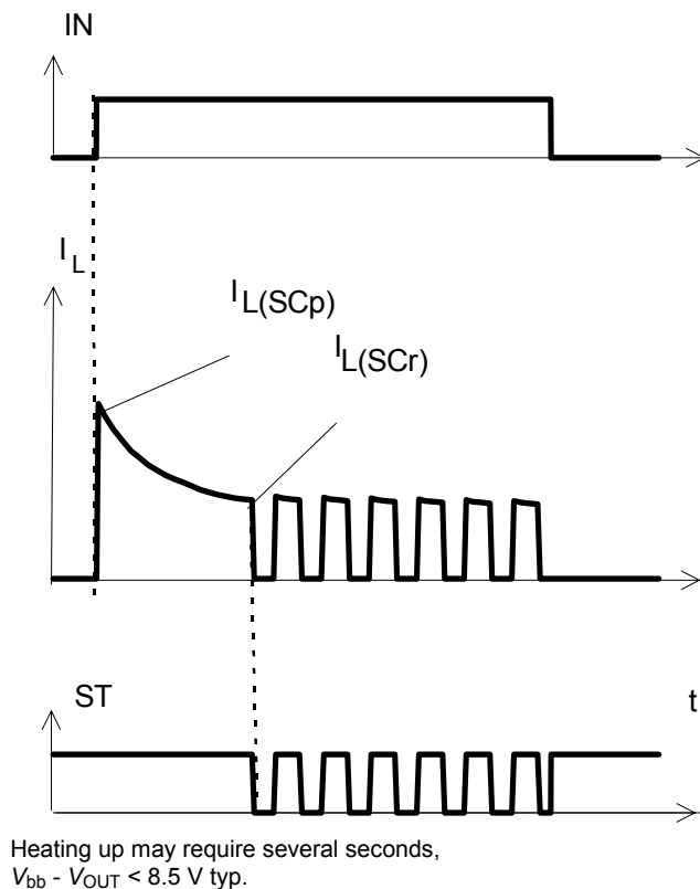
Figure 3b: Turn on into overload,
