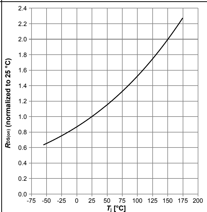
Diagram 10: Normalized drain-source on resistance
