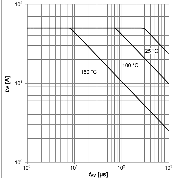
Diagram 14: Avalanche characteristics
