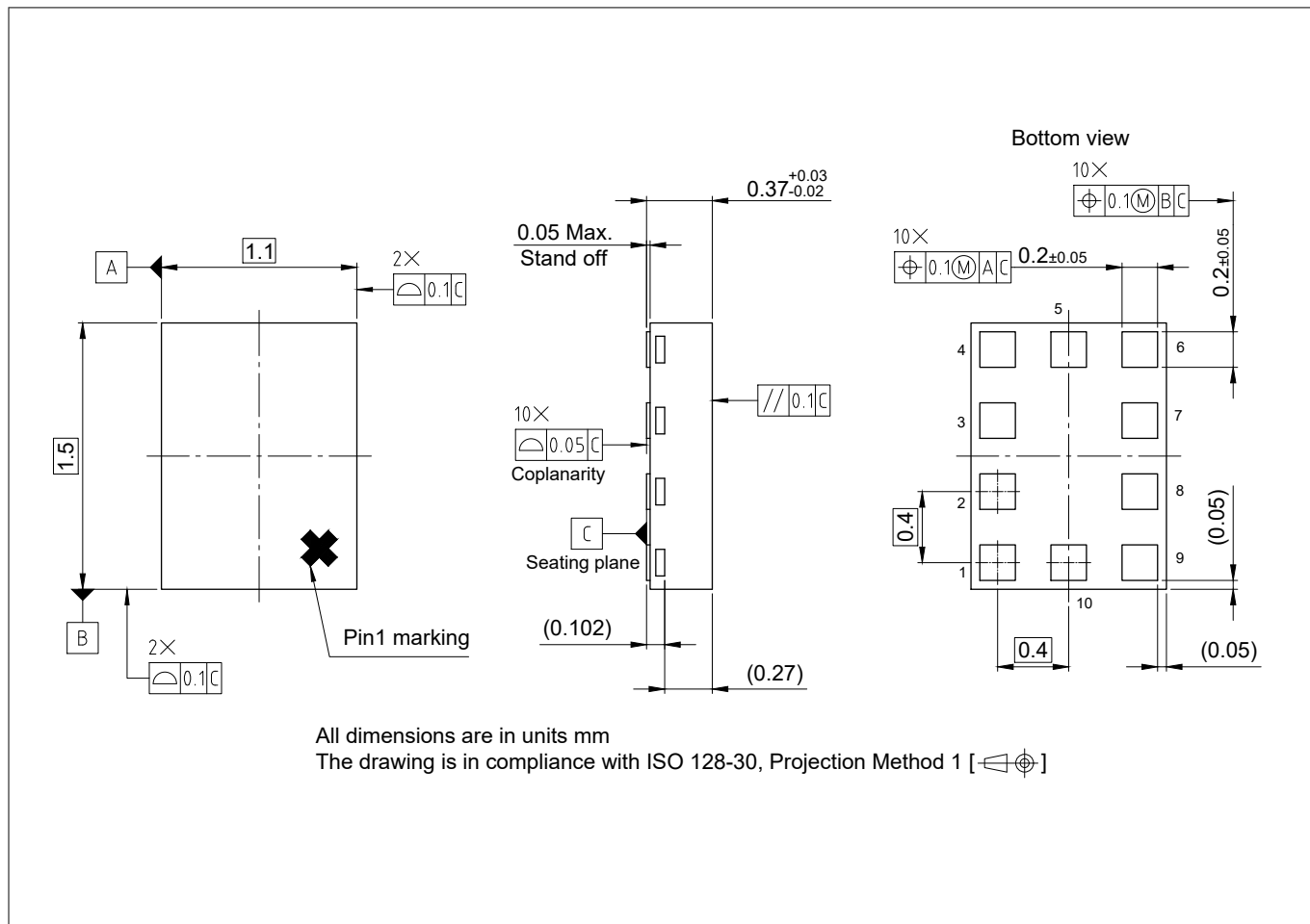
Figure 4 Package dimensions
