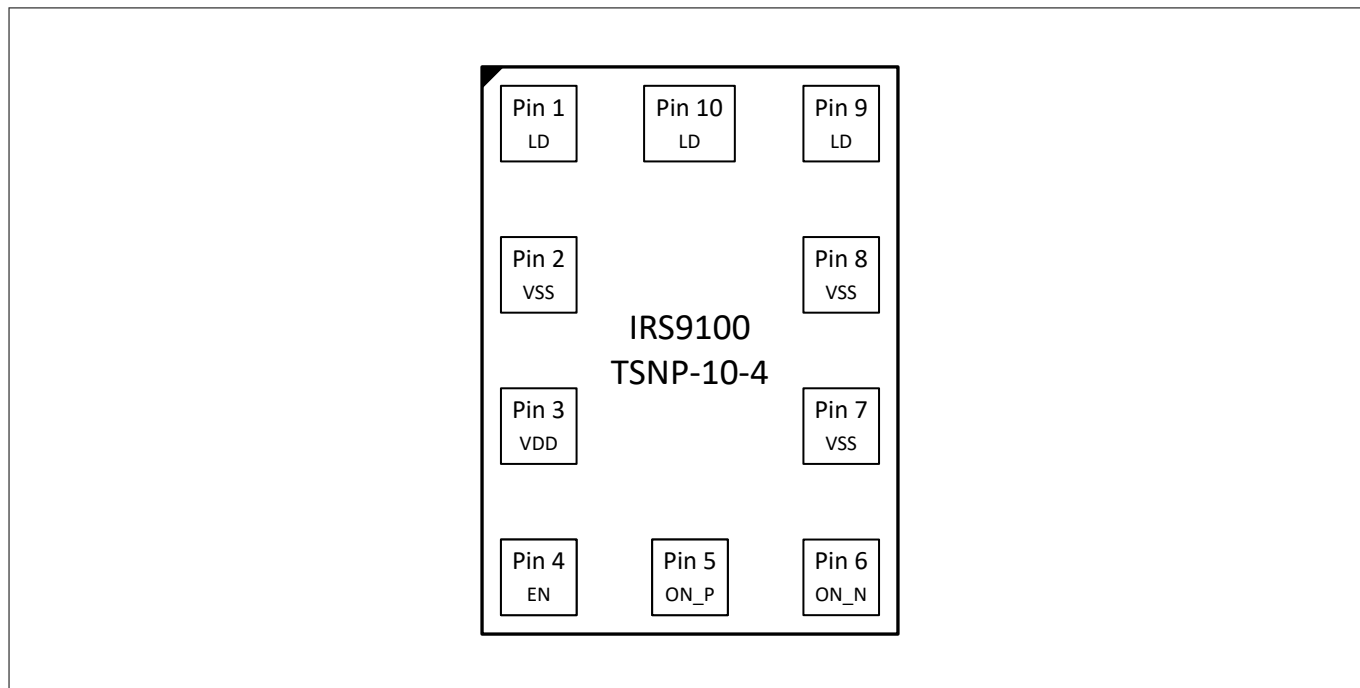
Figure 3 Pin-out
