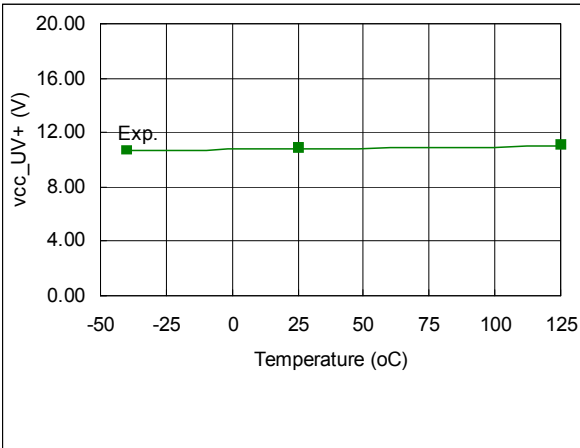
Figure 50: V_{CCUV+} vs. temperature
