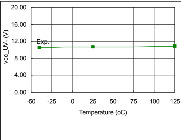
Figure 51: V_{CCUV-} vs. temperature
