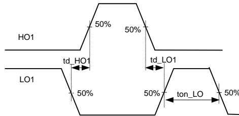
Deadtime Waveform
