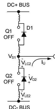
Figure 27: V_S negative
