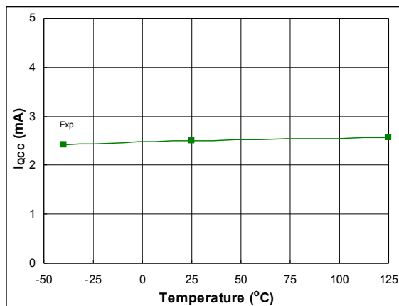
Figure 48: I_{QCC} vs. temperature
