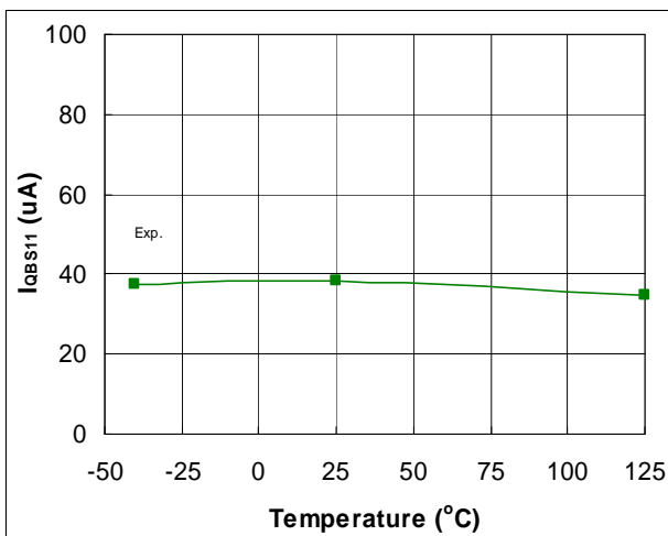
Fig. 37. Quiescent VBS Supply Current vs. Temperature
