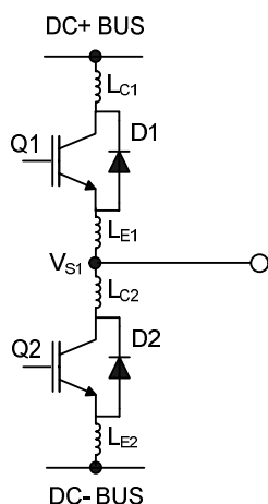
Figure 19: Parasitic Elements
