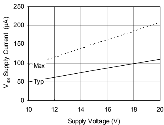
Figure 12B. V BS Supply Current vs. Supply Voltage
