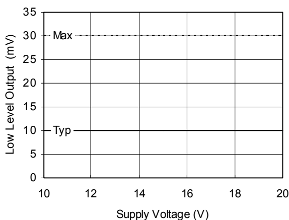
Figure 10B. Low Level Output vs. Supply Voltage ( I_O = 2 mA)
