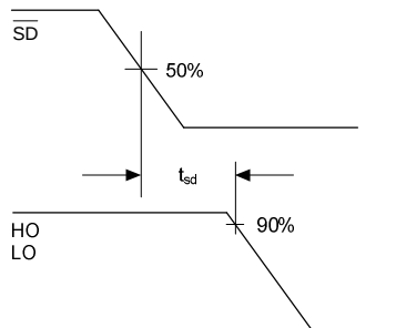
Figure 3: Shutdown Waveform Definitions
