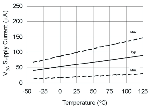
Figure 19A. V BS Supply Current vs. Temperature
