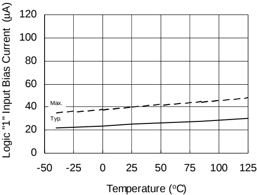
Figure 15A. Logic "1" Input Bias Current vs. Temperature
