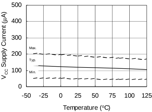
Figure 14A. V_{CC} Supply Current vs. V_{CC} Temperature
