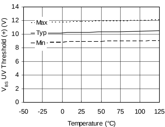
Figure 25A. V_{BS} UV Threshold (+) vs. Temperature
