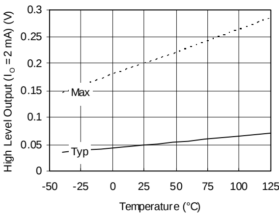
Figure 16A. High Level Output ( I_o = 2\text{ mA} ) vs. Temperature
