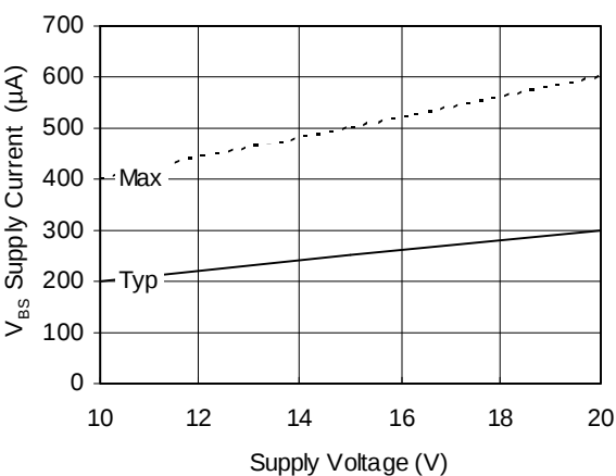
Figure 19B. V BS Supply Current vs. Voltage
