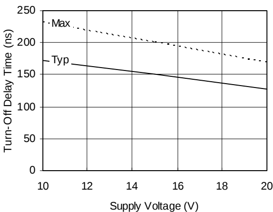
Figure 7B. Turn-Off Delay Time vs. Voltage
