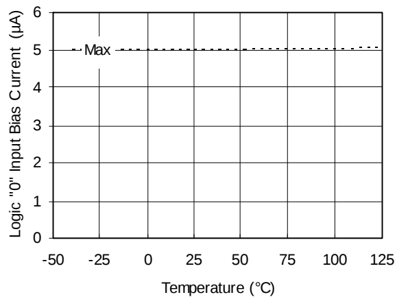
Figure 22A. Logic "0" Input Bias Current vs. Temperature
