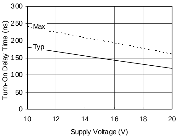
Figure 6B. Turn-On Delay Time vs. Voltage
