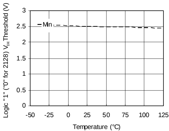
Figure 13A. Logic "1" ("0" for 2128) V_{IH} Threshold vs. Temperature
