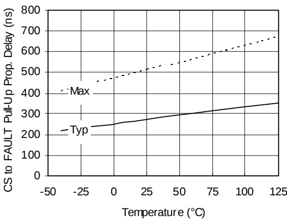
Figure 12A. CS to FAULT Pull-Up Prop. Delay vs. Temperature
