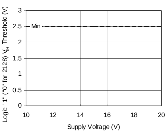
Figure 13B. Logic "1" ("0" for 2128) V_{IH} Threshold vs. Voltage
