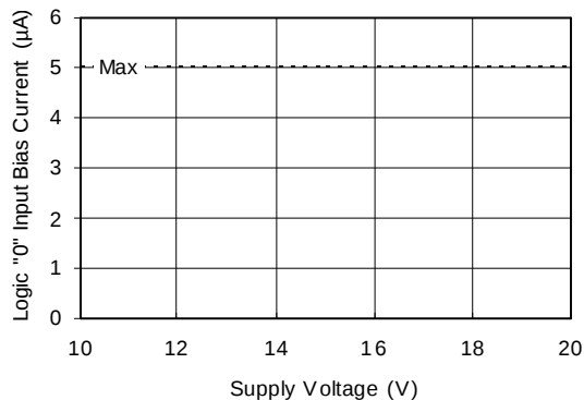
Figure 17B. Logic "0" Input Current vs. Voltage
