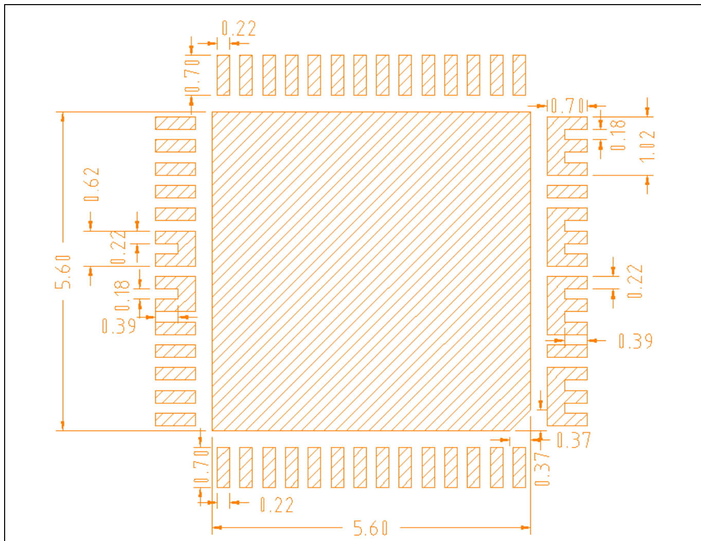
Figure 39 PCB PAD Size
