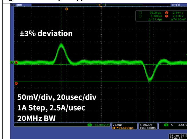
Figure 30 Transient response
