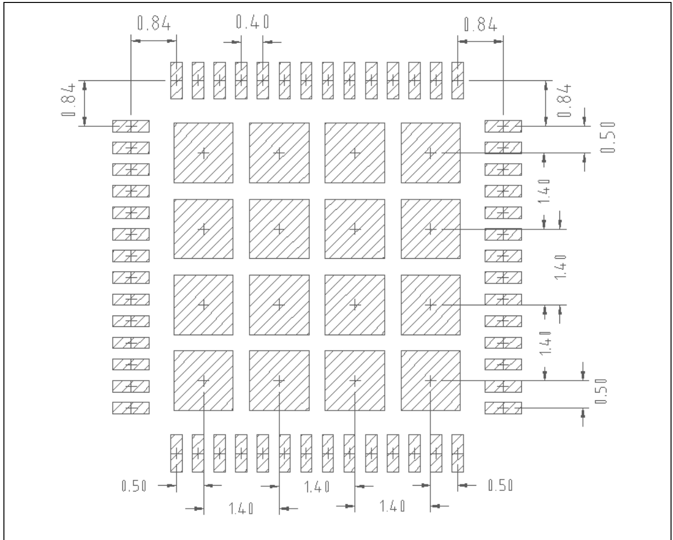
Figure 42 Solder paste stencil pad spacing
