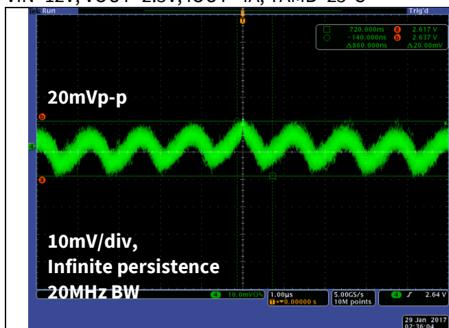
Figure 28 Output ripple
