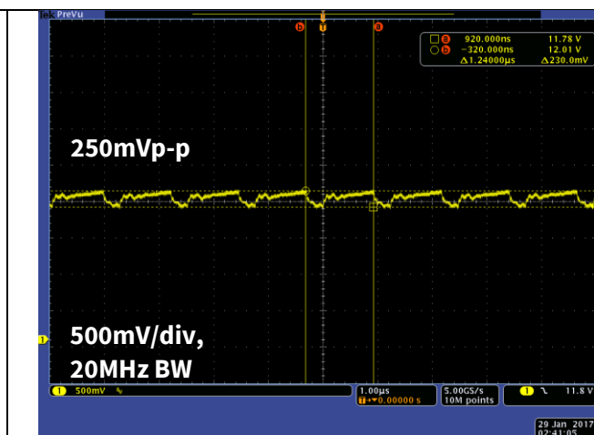
Figure 29 Input ripple
