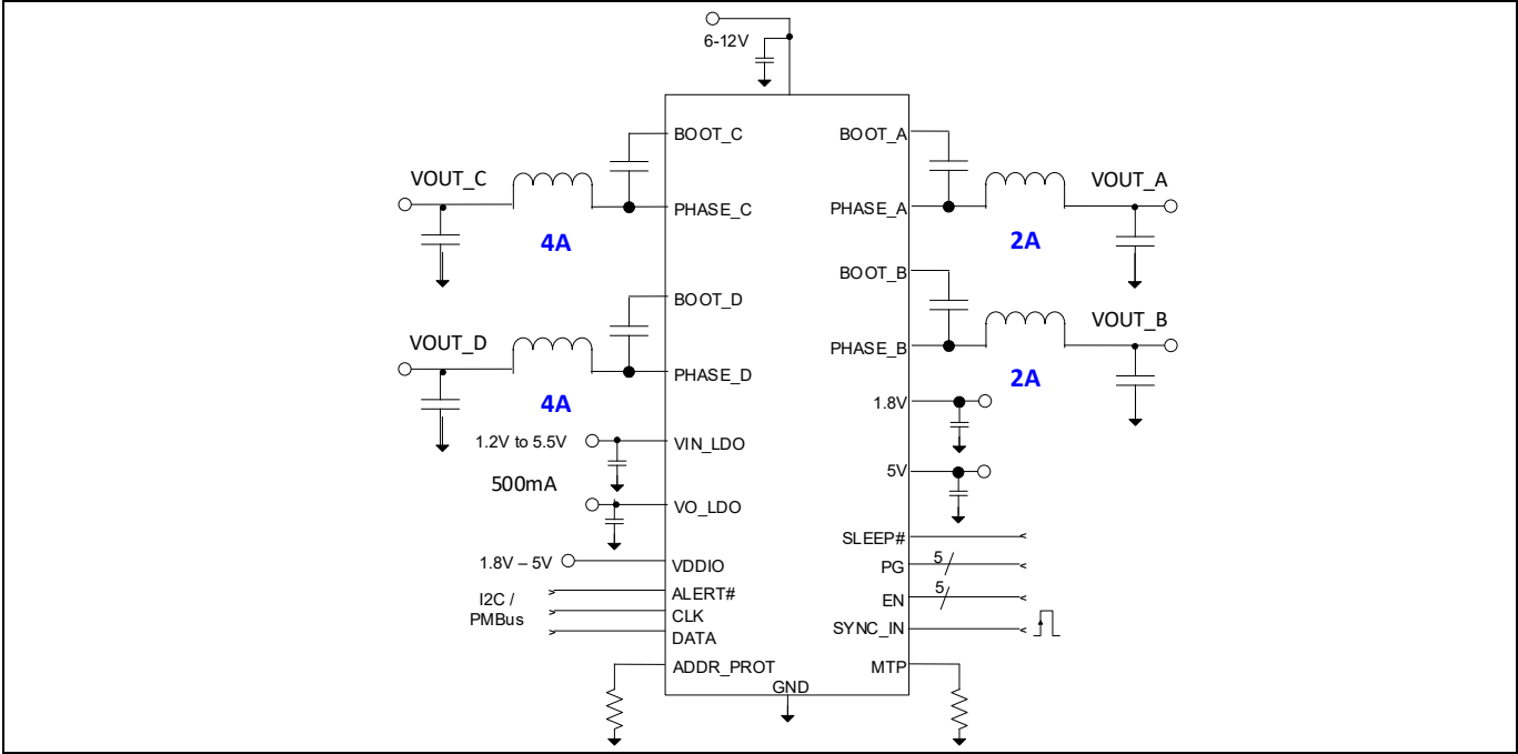
Figure 1 IRPS5401 Basic application circuit
