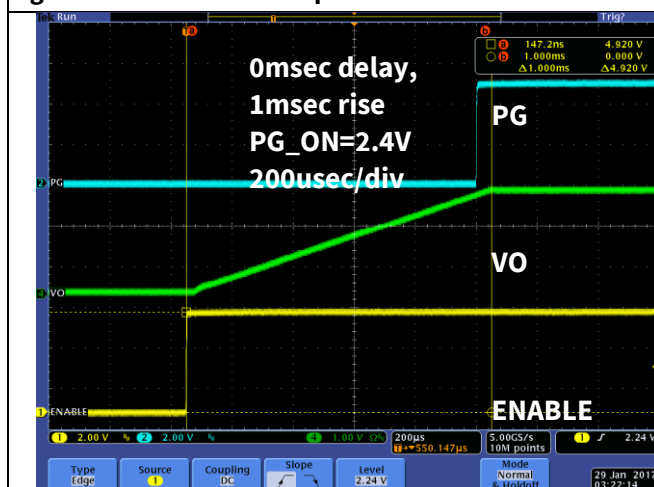
Figure 32 Enable start
