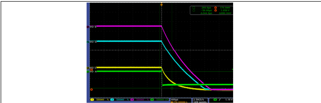
Figure 18 Global_fault_en=1
