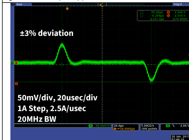
Figure 30 Transient response
