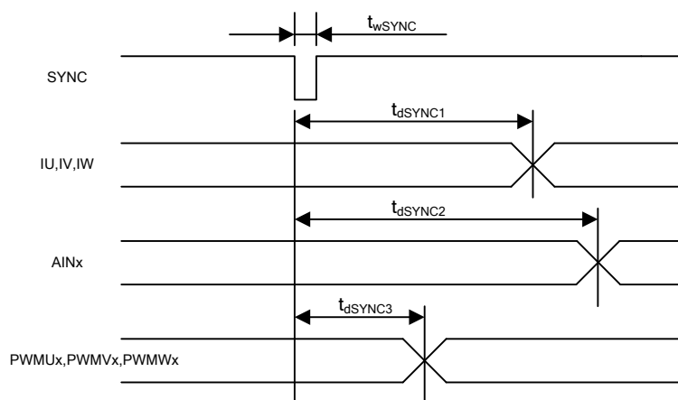
Figure 9. SYNC timing
