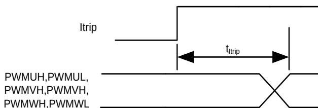
Figure 11. ITRIP timing
