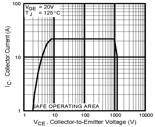
Fig. 12 - Turn-Off SOA
