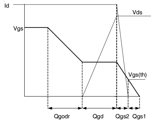
Fig 18b. Gate Charge Waveform
