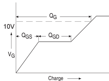
Fig 12b. Basic Gate Charge Waveform
