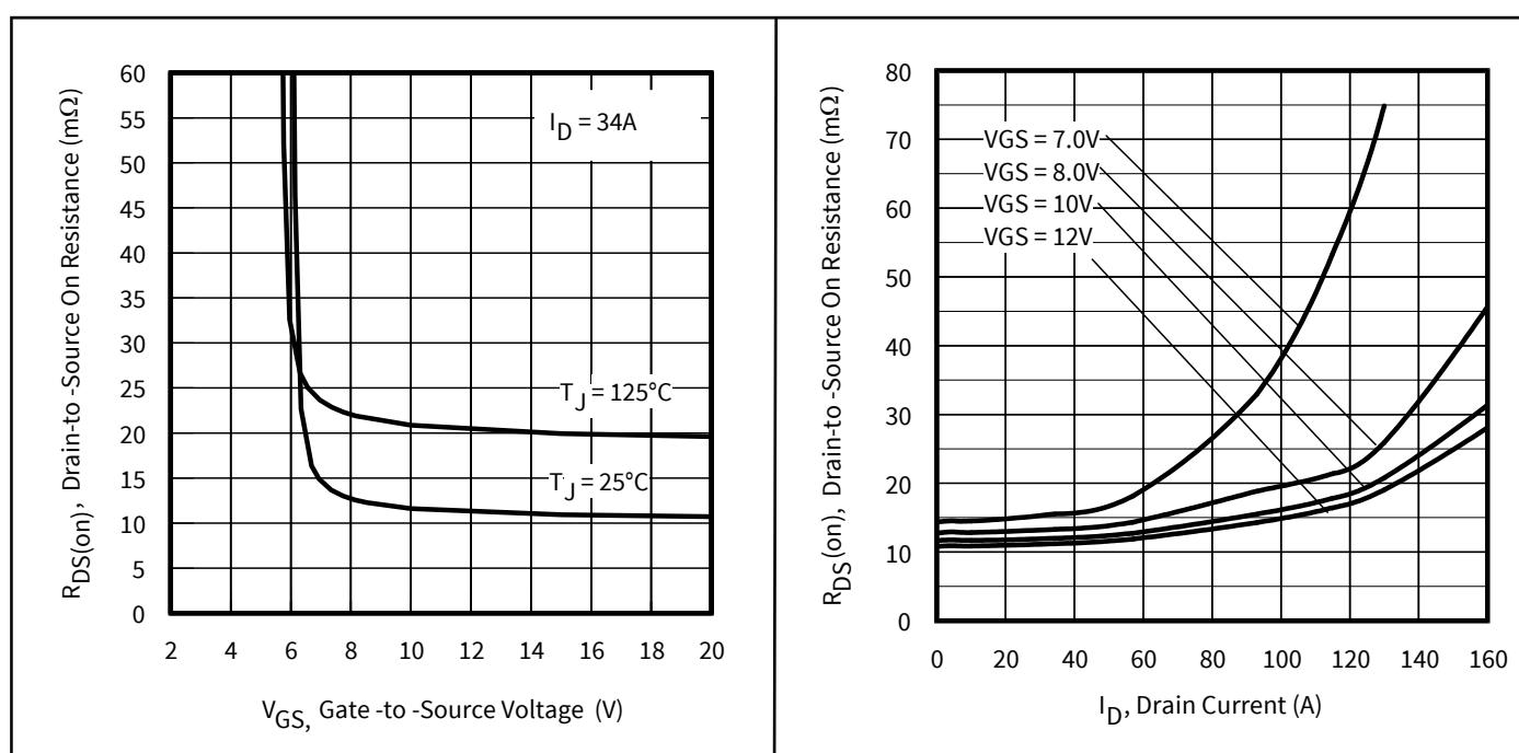
Figure 1 Typical On-Resistance vs. Gate Voltage
