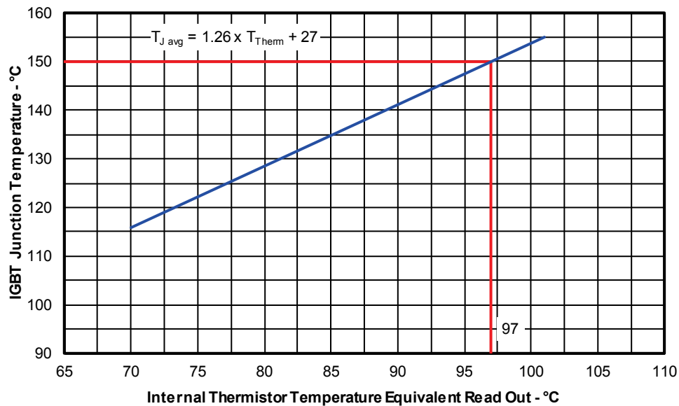
Figure 9. Estimated Maximum IGBT Junction Temperature vs. Thermistor Temperature Sinusoidal Modulation, V^+ = 400\text{V} , I_{phase} = 7.5\text{Arms} , f_{sw} = 16\text{kHz} , f_{mod} = 50\text{Hz} , MI = 0.8 , PF = 0.6
