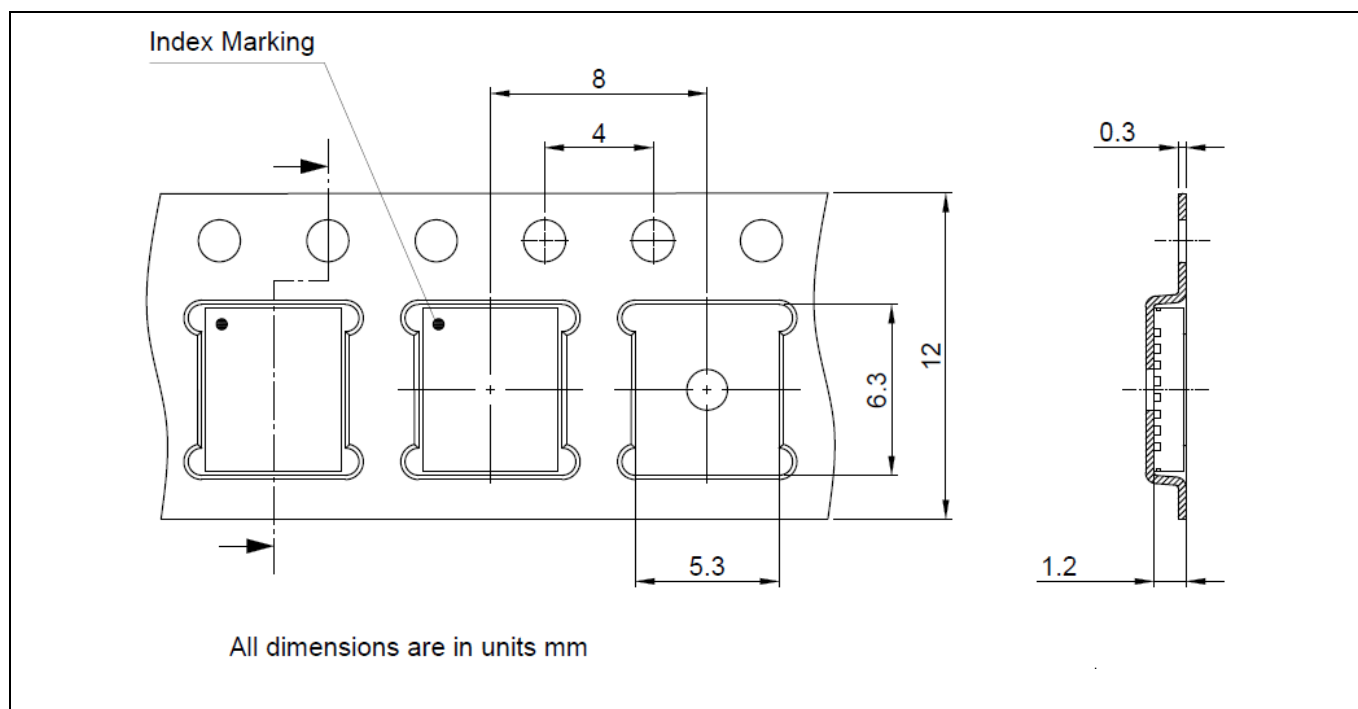
Figure 35 Pin 1 orientation in the tape
