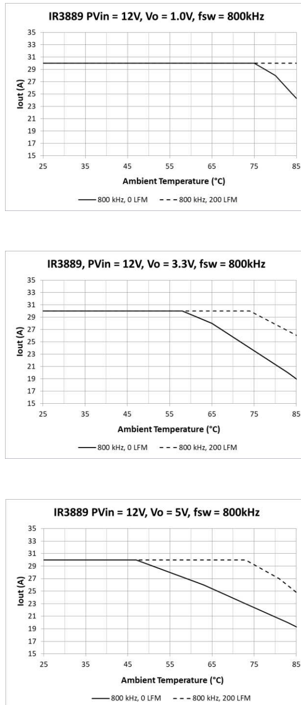
Figure 4 Thermal de-rating curves, P_{Vin} = 12V , V_o = 1.0V/3.3V/5V , F_{sw} = 800kHz , V_{CC} = \text{Internal LDO}
