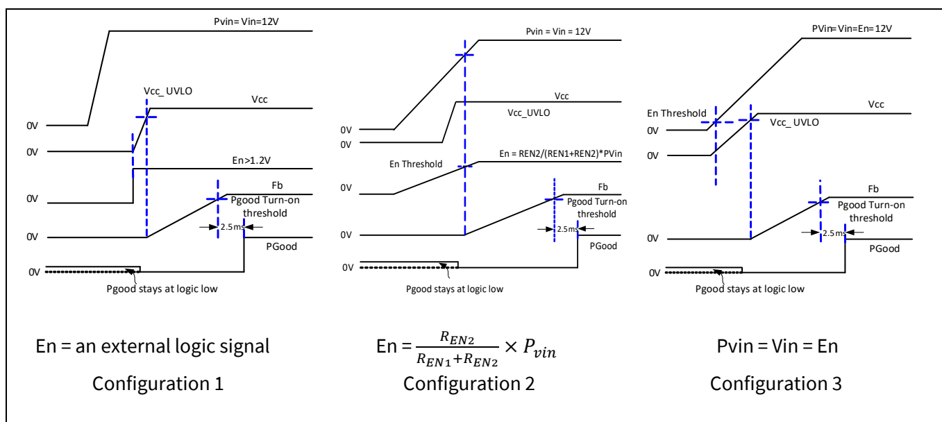
Figure 10 Start-up sequence
