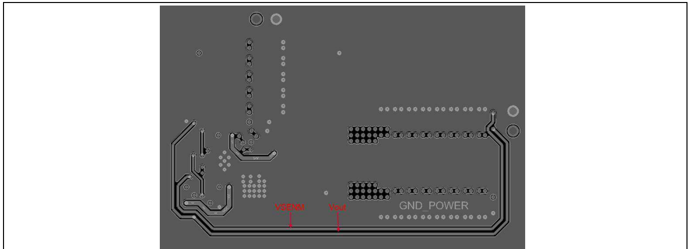
Figure 27 IR3888 Demo Board – 3 rd Layer (Ground & Signal)
