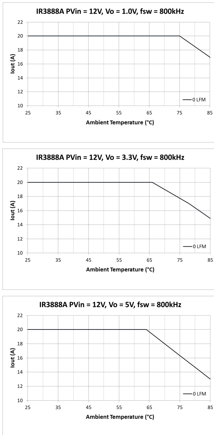
Figure 4 Thermal de-rating curves, P_{Vin} = 12V , V_{out} = 1.0V/3.3V/5V , f_{sw} = 800kHz , VCC = Internal LDO
