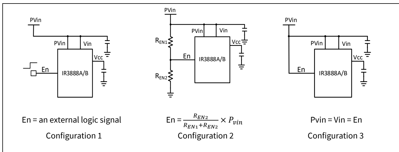
Figure 8 Enable Configurations
