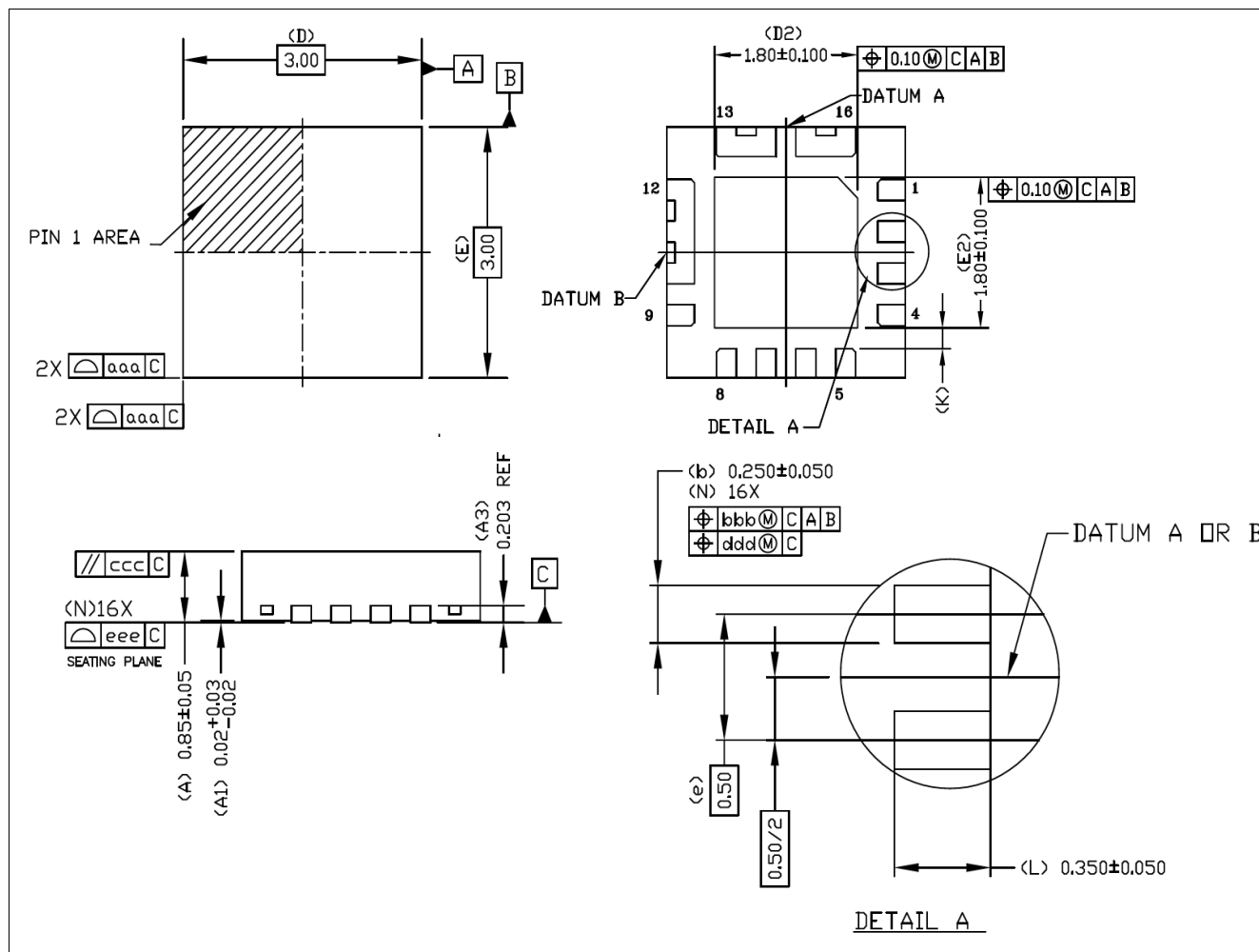
Figure 8-8 Package Dimensions
