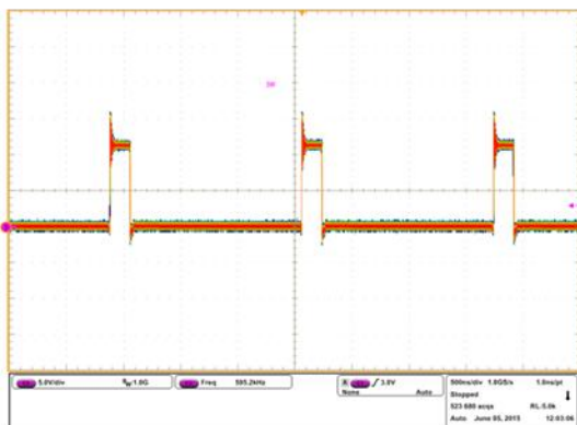
Figure 45: Inductor node at 15A load Ch 3 :SW node
