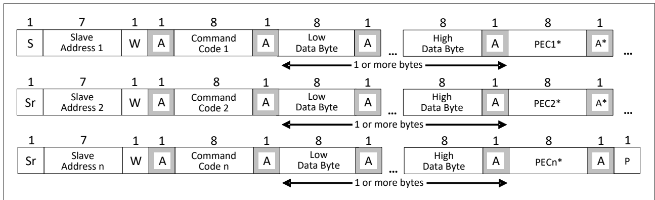
Figure 64: Group Command
