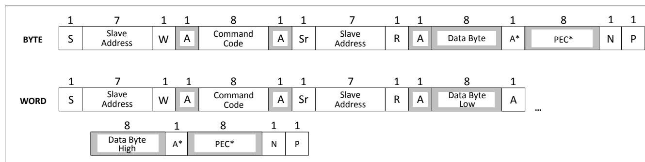
Figure 59: SMBus Read Byte/Word
