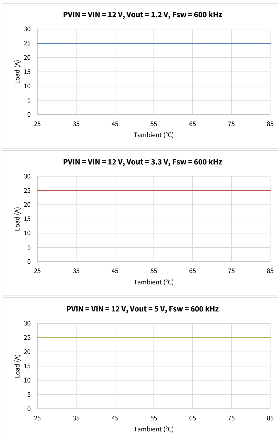
Figure 4 Thermal derating curves, PVIN = 12 V, Vout = 1.2 V/3.3 V/5 V, fsw = 600 kHz, VCC = Internal LDO
