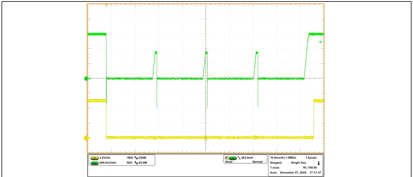
Figure 18 Short circuit and UVP (Hiccup), (Ch1: PGGood, Ch4: Vo)
