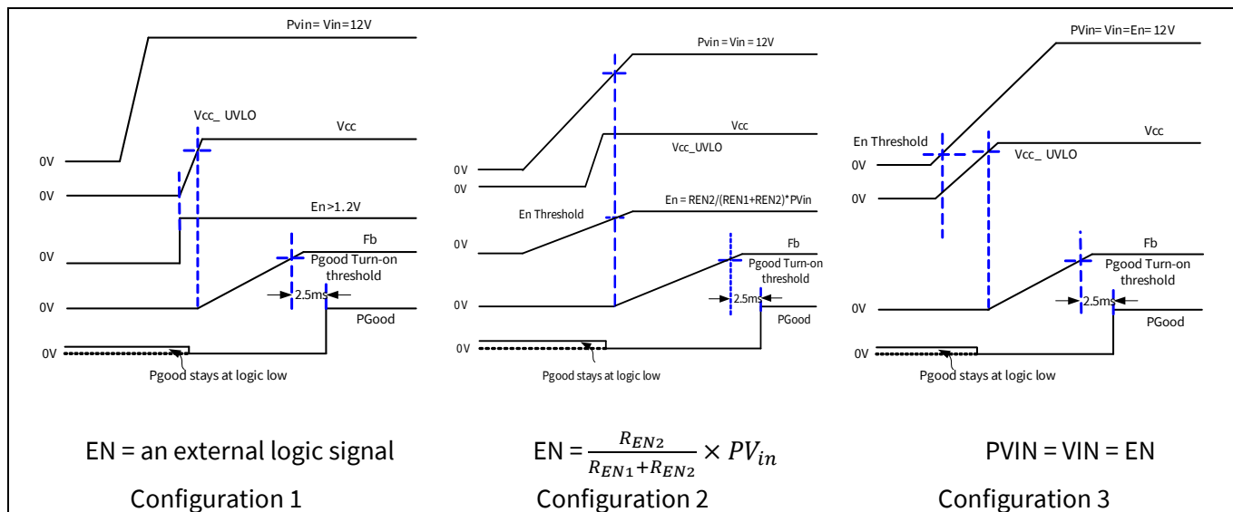
Figure 8 Start-up sequence
