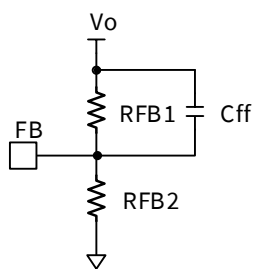
Figure 12 Configuration of feedforward capacitor, Cff.
