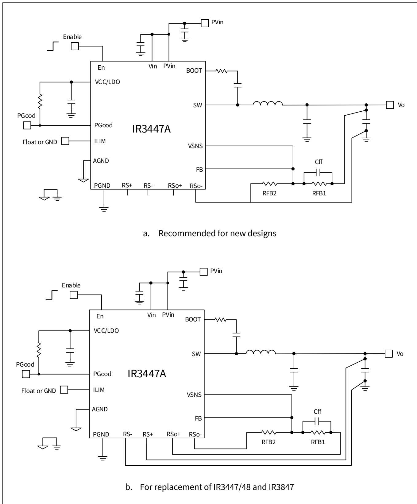
Figure 3 IR3447A basic application circuit
