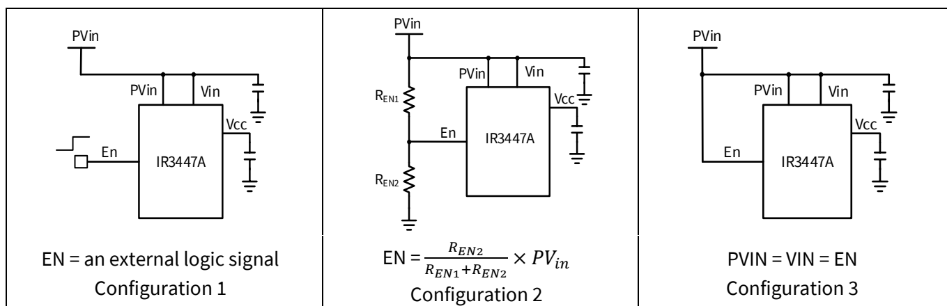
Figure 7 Enable Configurations
