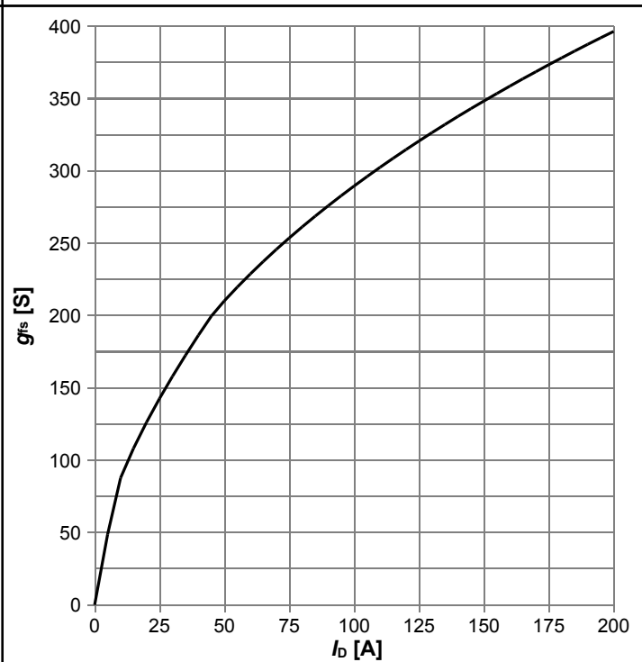
Diagram 8: Typ. transconductance
