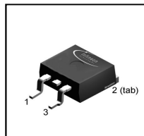
PG-TO263-3-2
