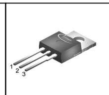
PG-TO220-3-1
