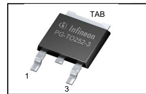
PG-TO252-3-313
