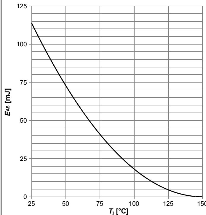
Diagram 12: Avalanche energy
