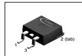
PG-TO263
