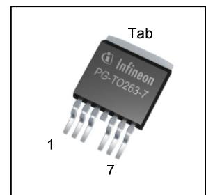
PG-TO263-7-3
