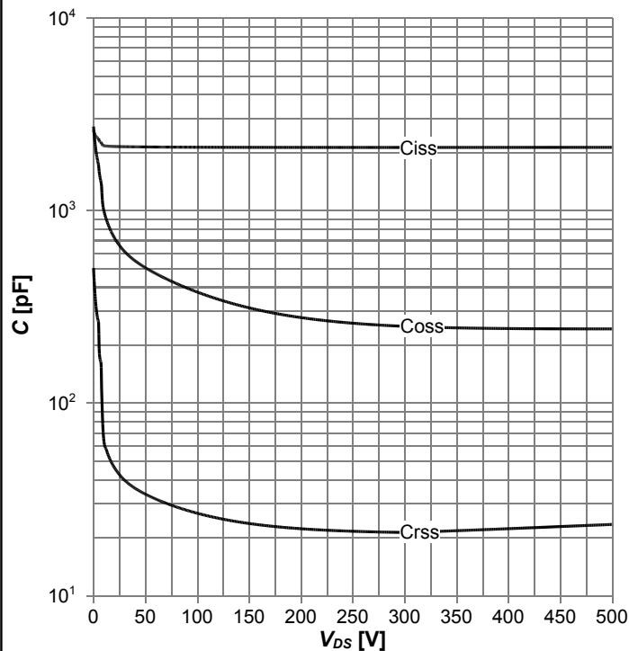
Diagram 15: Typ. capacitances
