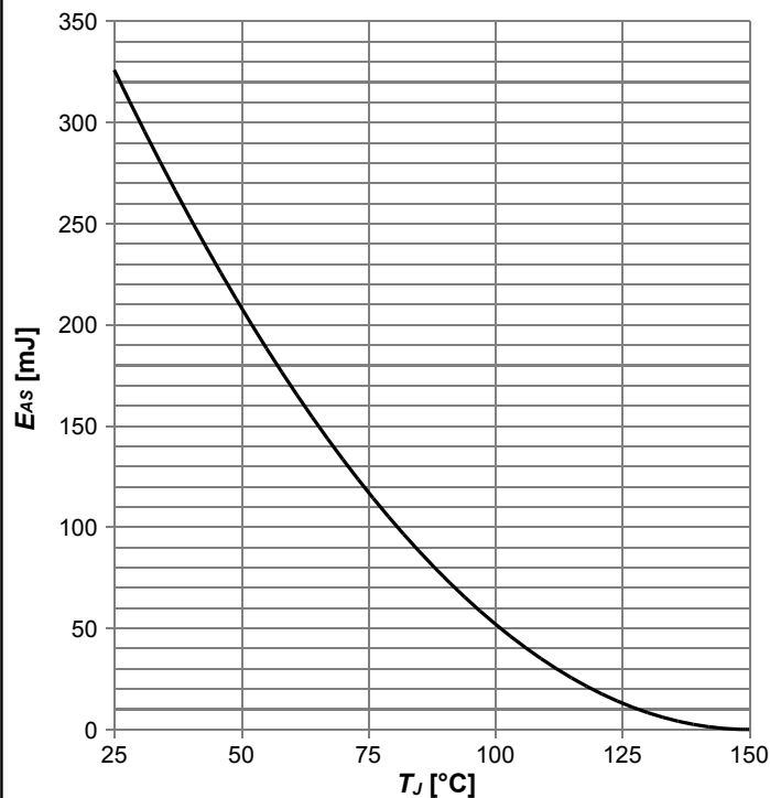
Diagram 13: Avalanche energy
