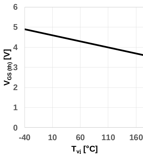
Figure 6 Typical gate-source threshold voltage as a function of junction temperature ( V_{GS(th)} = f(T_{vj}) , I_{DS} = 2.5mA , V_{GS} = V_{DS} )
